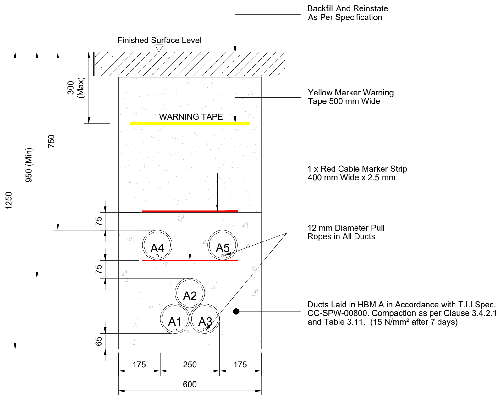
A=125 mm: Outer Diameter HDPE ESB Approved Duct, SDR=17.6 All Dimensions in Millimetres.
